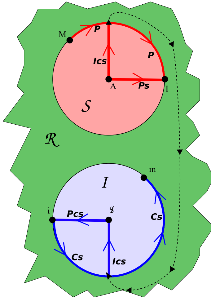
FIGURE 4.1. The disk
