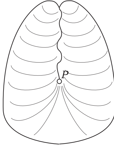
FIGURE 2.1. The cross-cap
