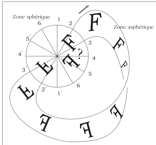
FIGURE 2.3. The projective plane
