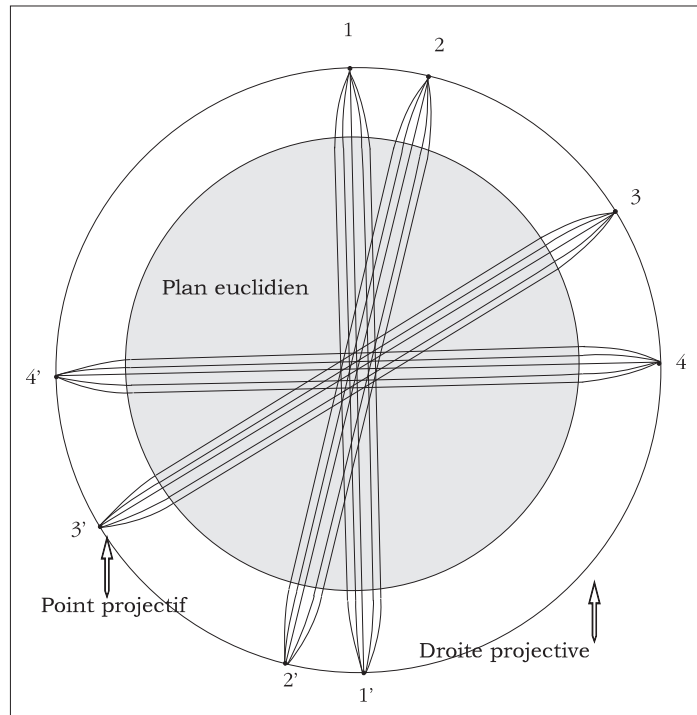
FIGURE 2.3. The projective plane
