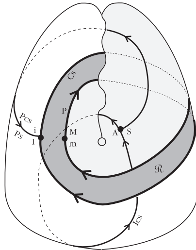
FIGURE 2.2. The R Schema imprinted on a cross-cap
